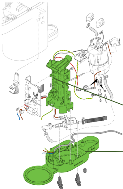
FIGURE 17: RECYCLED PLASTICS (IN FRAME AND BASE PLATE) IN THE SENSEO UP (SOURCE: PHILIPS)
