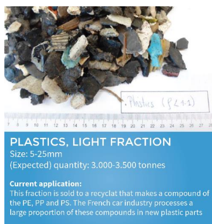
FIGURE 4: EXAMPLE OF LIGHT FRACTION PLASTICS IN SEPARATION FROM CAR WRECKS (SOURCE: ARN)
